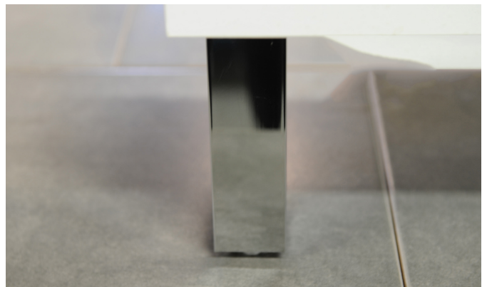
Square Leg. Height = 150mm - 166mm. Legs can be adjusted within this size.
